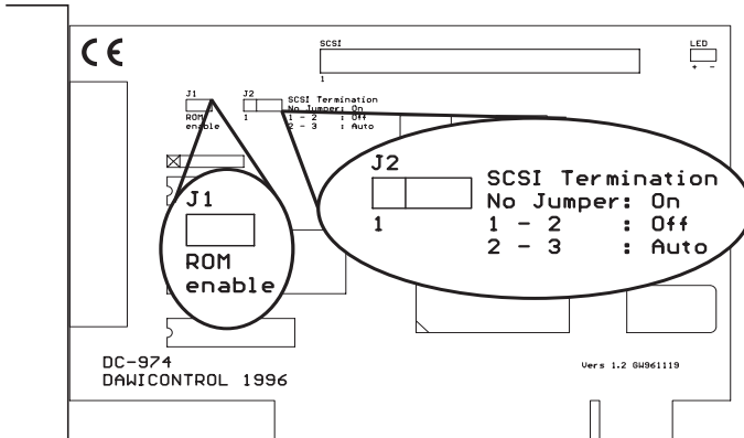
Skizze: DC-2974 PCI
