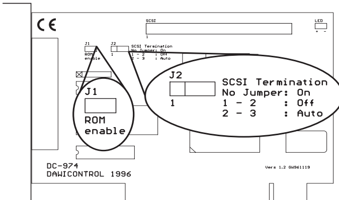
Figure: DC-2974 PCI
